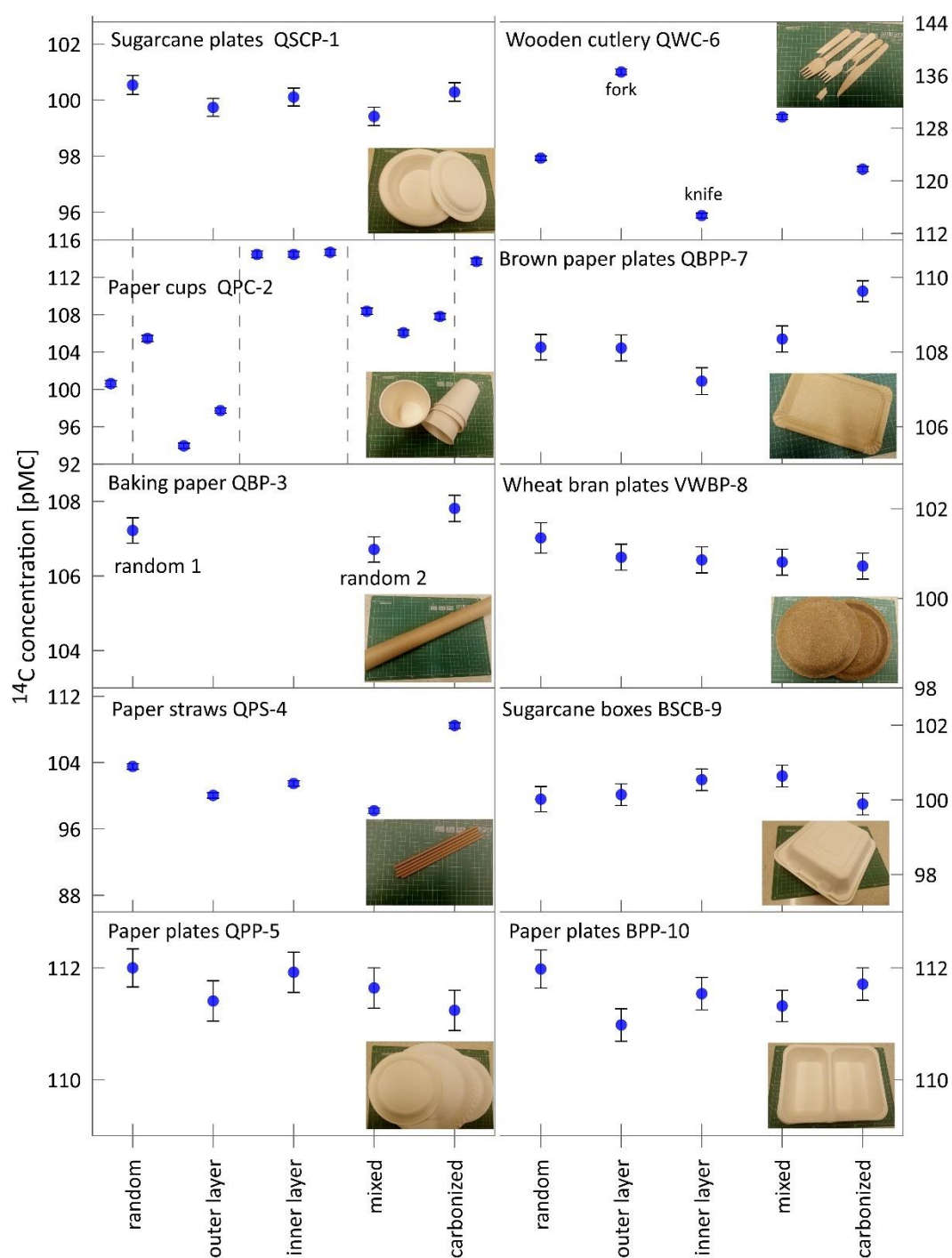
Fig. 6 Comparison of the ^{14}\text{C} isotope measurements of DPMs by AMS. (see Fig. 1 in (Gill et al. 2024)).
