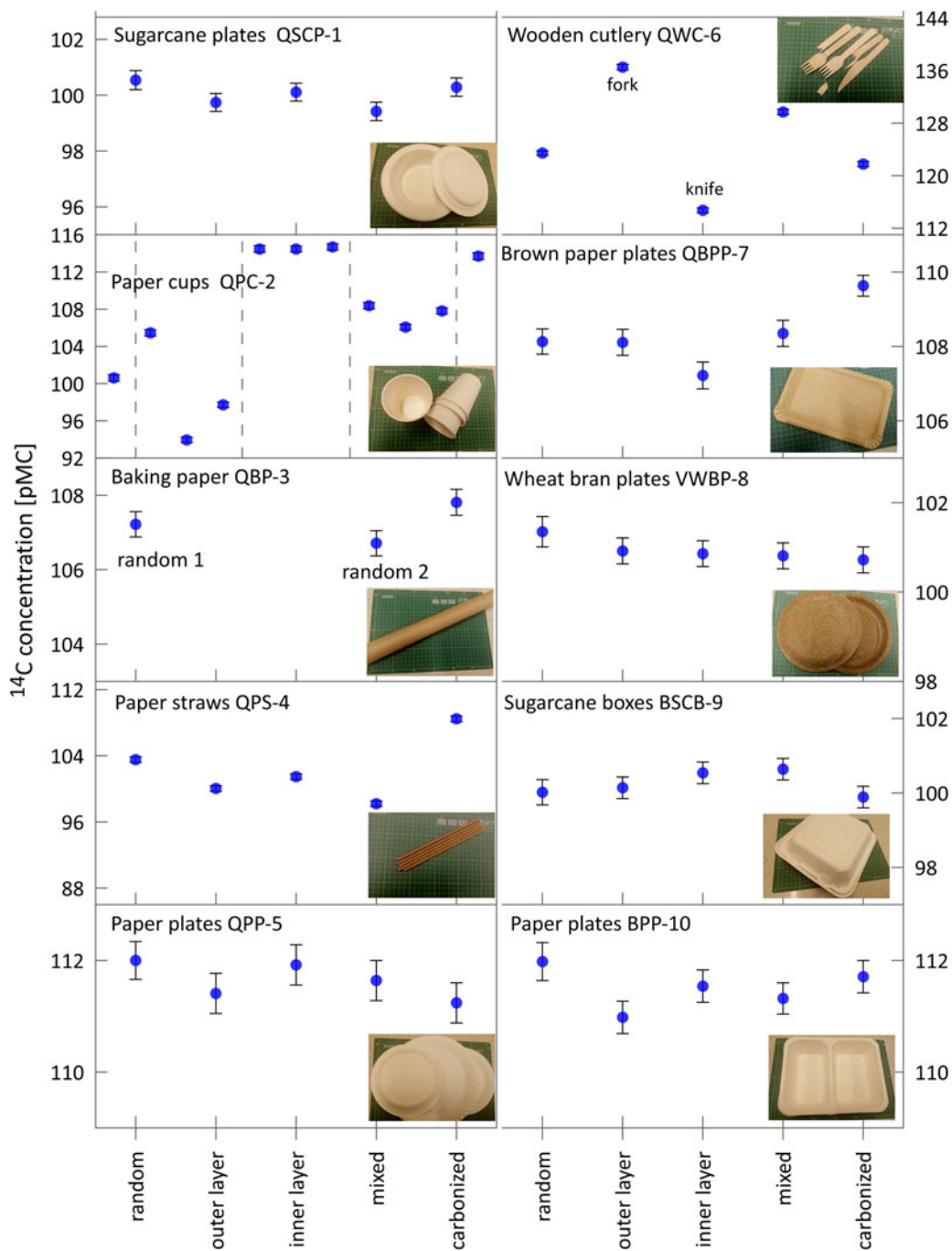
Figure 1 Comparison of the ^{14}\text{C} isotope measurements (see Supplementary Material).
