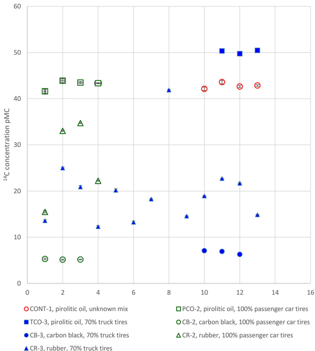
Figure 2 Comparison of the ^{14}\text{C} isotope measurements. Measurement uncertainties are smaller than the size of the symbols used.
