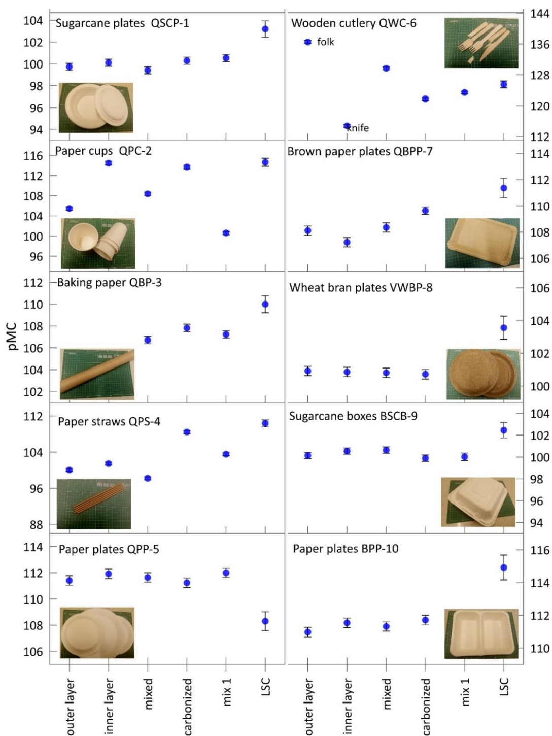
Fig. 8 Comparison of the ^{14}\text{C} concentration measurements of DPMs by LSC and AMS.
